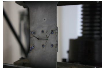
图7 裂纹试件拉伸破坏试验 Fig.7 Crack specimen failure test
