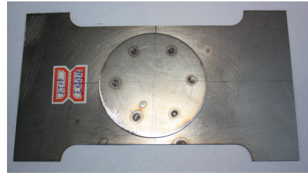
图6 破孔点焊修补试件 Fig.6 Spot welding repair specimen for broken hole
