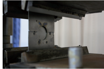
图8 破孔试件拉伸破坏试验 Fig.8 Broken hole specimen failure test
